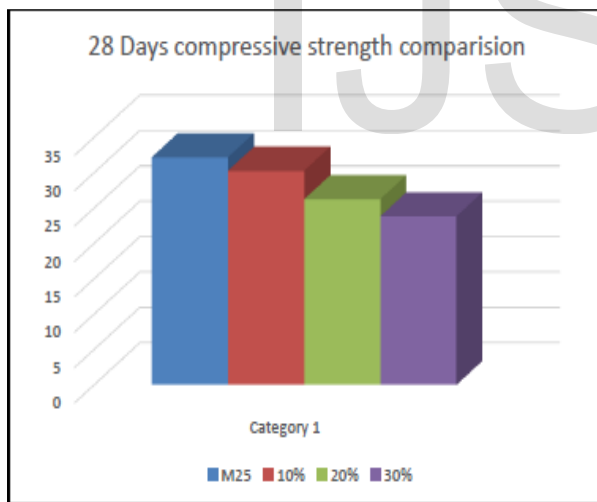
Fig. No. 3.4 Graph for 28 Days Compressive Strength Comparison
