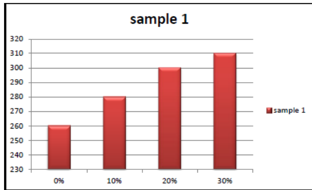
Fig. No. 3.3 Results of Slump Cone Test
